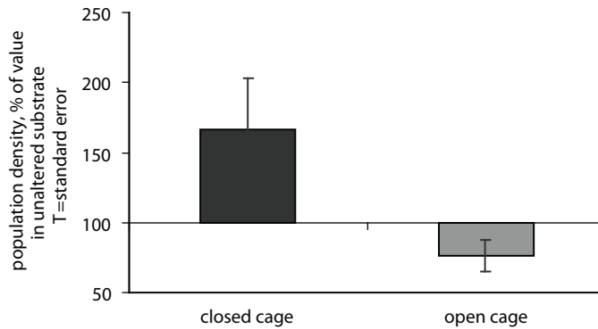
Fig. 5. Relative population density of Pyrgophorus coronatus in muddy/sandy substrate in Lake Apoyo, in closed exclusion cages and open exclusion cages at 10 m water depth. Values given are relative to population density in unaltered sandy/muddy substrate. Standard errors of the mean shown for five observations (n=5).
