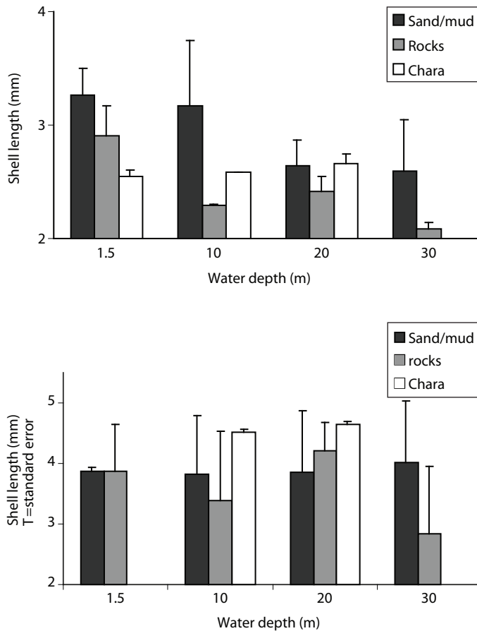
Fig. 4. Shell length of Pyrgophorus coronatus at varying water depths according to habitat type in Lake Xilola (A) and in Lake Apoyo (B). Standard errors of the mean shown for the following sample sizes at each respective lake and depth: Xilola-sand/mud, 1.5 m, n=10; 10 m, n=5; 20 m, n=24; 30 m, n=7; Xilola-rocks, 1.5 m, n=14; 10 m, n=48; 20 m, n=41; 30 m, n=46; Xilola-Chara, 1.5 m, n=339; 10 m, n=308; 20 m, n=118; Apoyo-sand/mud, 1.5 m, n=69; 10 m, n=72; 20 m, n=137; 30 m, n=24; Apoyo rocks, 1.5 m, n=9; 10 m, n=17; 20 m, n=61, 30 m, n=6; Apoyo-Chara, 10 m, n=345; 20 m, n=129.
