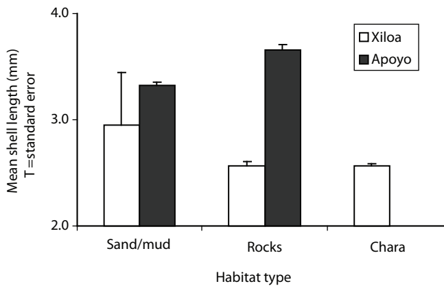
Fig. 2. Shell length of Pyrgophorus coronatus at 1.5 m depth, by habitat in Lake Xilola and Lake Apoyo. Standard errors of the mean shown for the following numbers of individuals: Xilola-sand/mud, n=4; rocks, n=285; Chara, n=1 779; Apoyo-sand/mud, n=699; rocks, n=549.
