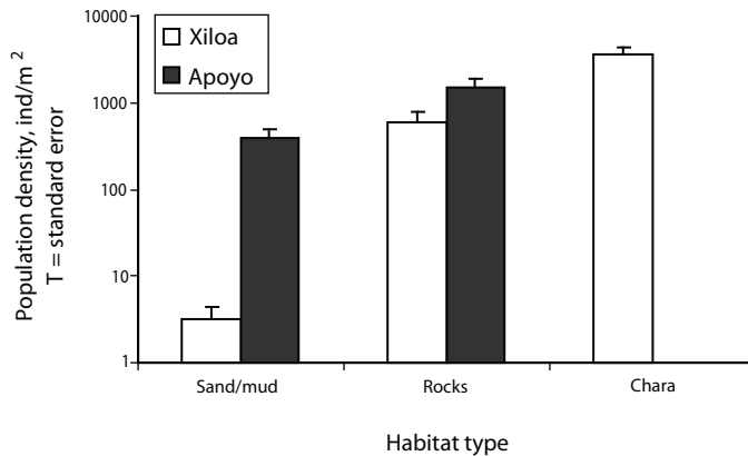
Fig. 1. Population density of Pyrgophorus coronatus at 1.5 m depth, by habitat, in Lake Xilola and in Lake Apoyo. Standard errors of the mean shown for twelve monthly measurements (n=12).
