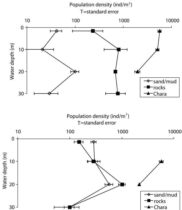
Fig. 3. Population density of Pyrgophorus coronatus at varying water depths according to habitat type in Lake Xiloa (A) and Lake Apoyo (B). Standard errors of the mean for three measurements shown (n=3).
